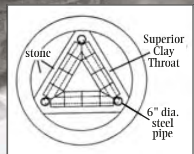
Triangular Fireplace
