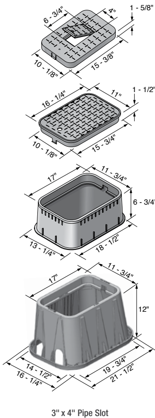
3" x 4" Pipe Slot
