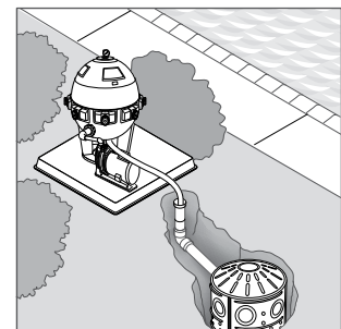
Backwash tank
